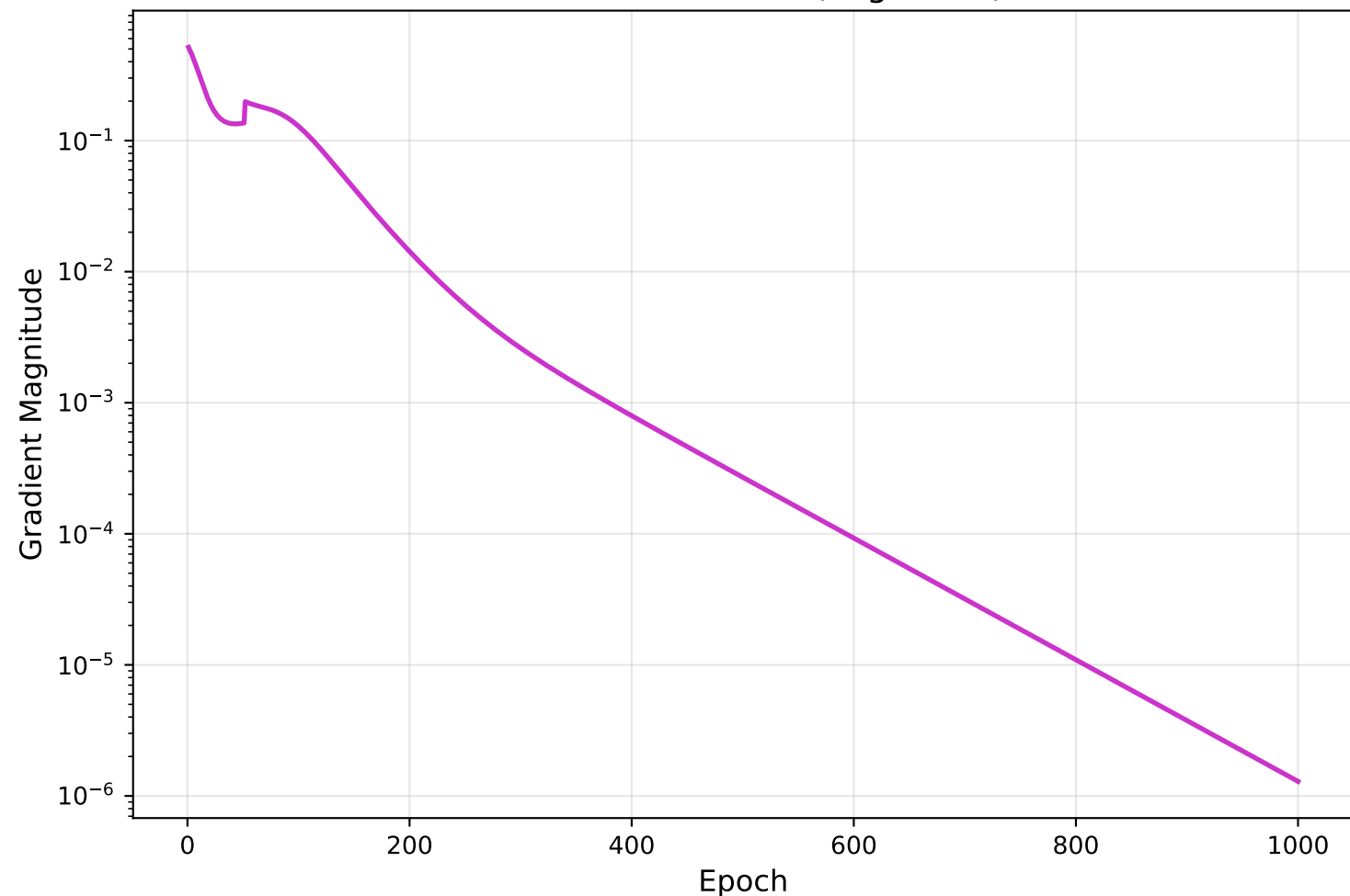
Optimization Dashboard
